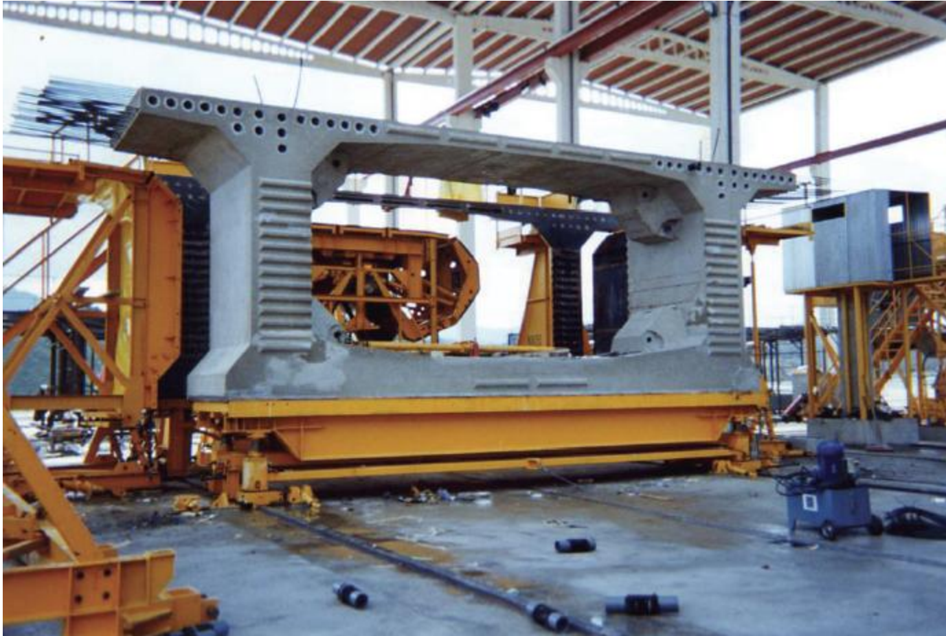
SHORT LINE MOULD WITH DOLLIES
